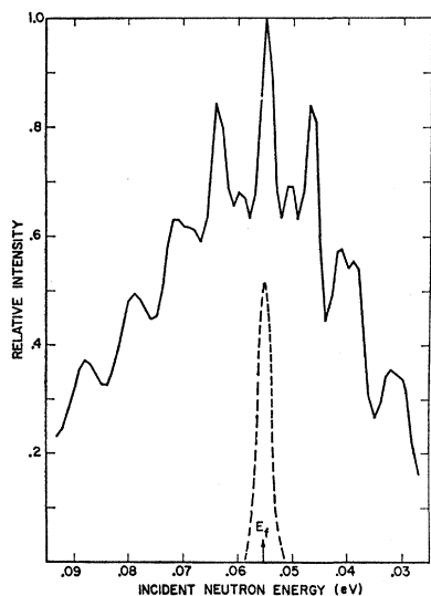
FIG. 1. Normalized energy distribution of neutrons scattered at 70° by water. Also shown is the resolution function (dashed curve).
