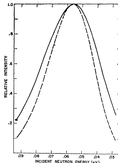
FIG. 3. Normalized energy distribution of neutrons scattered at 70^\circ by water assuming free translations (solid curve). Also shown is the curve for a mass 18 ideal gas with no internal degrees of freedom (dashed curve).
